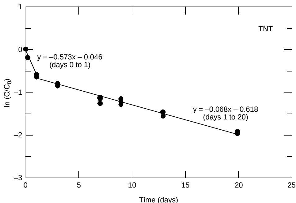
Figure 4. Plot of \ln(C/C_0) versus time (days) for TNT at room temperature ( 22 \pm 2^\circ\text{C} ) illustrating a multiple stage decay process.
