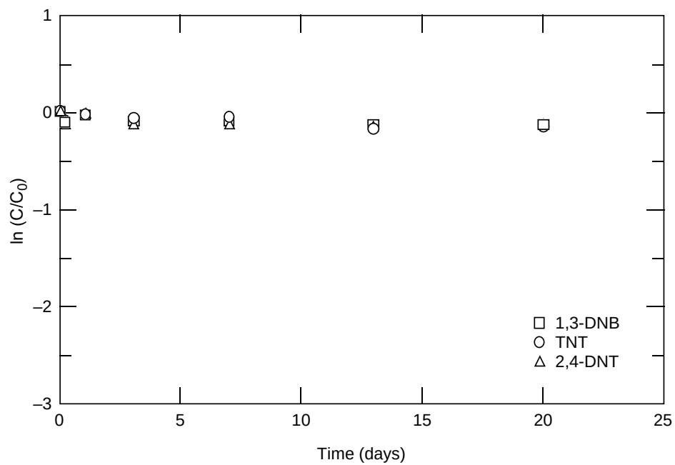
Figure 5. Plots of \ln(C/C_0) versus time (days) at the two lower temperatures.
