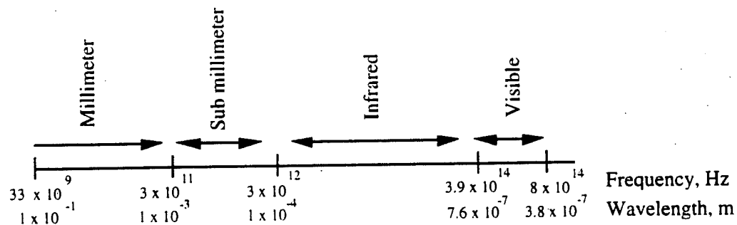
Figure 2.1.5.1. Electromagnetic Spectrum
