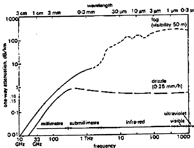
Figure 2.2.5.4. Attenuation of Electromagnetic Radiation as a Function of Wavelength
