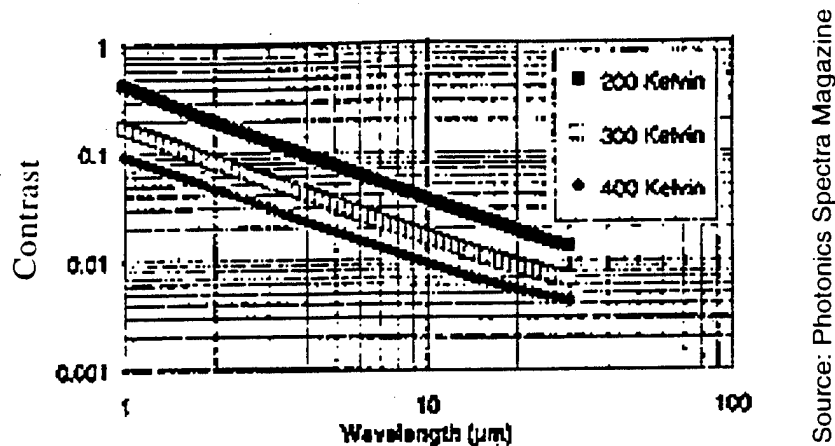
Figure 2.2.5.3. Contrast vs. Wavelength for Selected Temperatures
