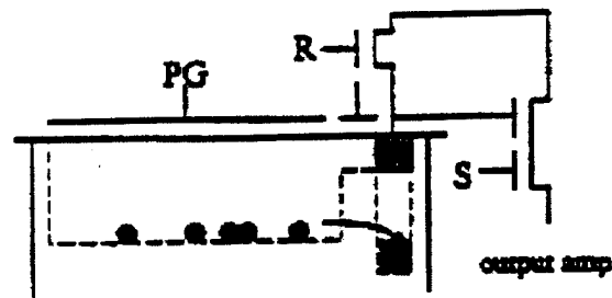
Figure 2.3.4.1 Schematic of an active pixel sensor (APS)
