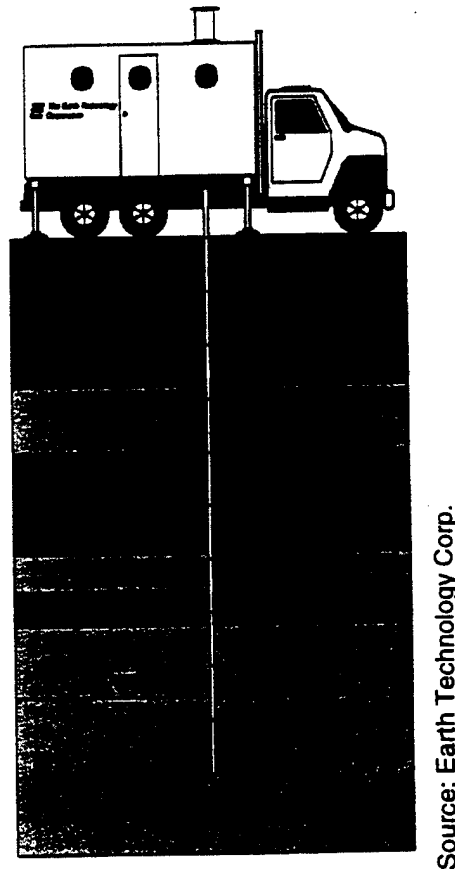
Figure 2.1.9.1 Example of Cone Penetrometer Operation
