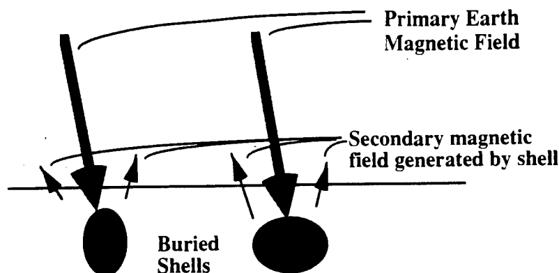
Figure 2.1.1.1 Secondary Magnetic Field Generated by Buried Ferromagnetic Shells
