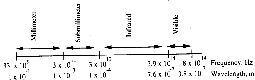
Figure 2.2.4.1 Electromagnetic Spectrum
