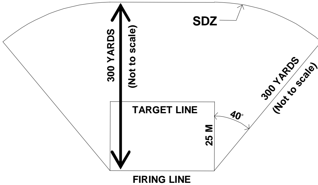
Figure 5. SDZ Requirement for Frangible Ammunition on a 25-Meter Partially Contained Range with Earth Side Berms and Earth Backstop
