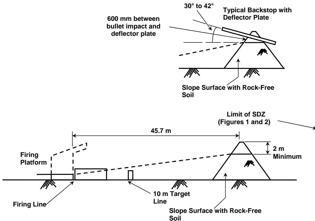
Figure 11. M60 Machine Gun, 10-Meter Tube Range Typical Cross-Section
