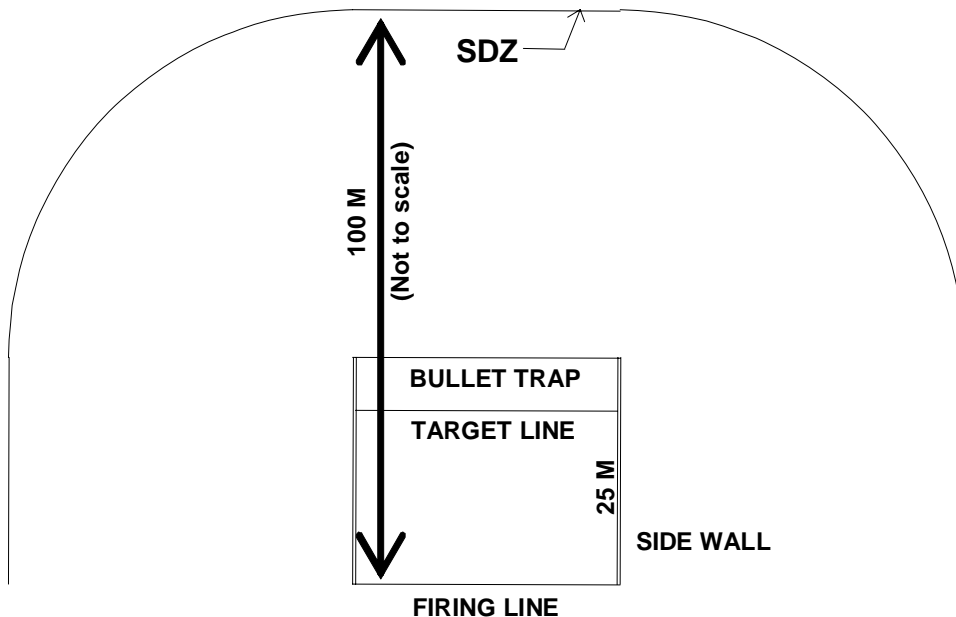
Figure 6. SDZ Requirements for Frangible Ammunition on a 25-Meter Partially Contained Range with Sidewalls and Bullet Trap.
