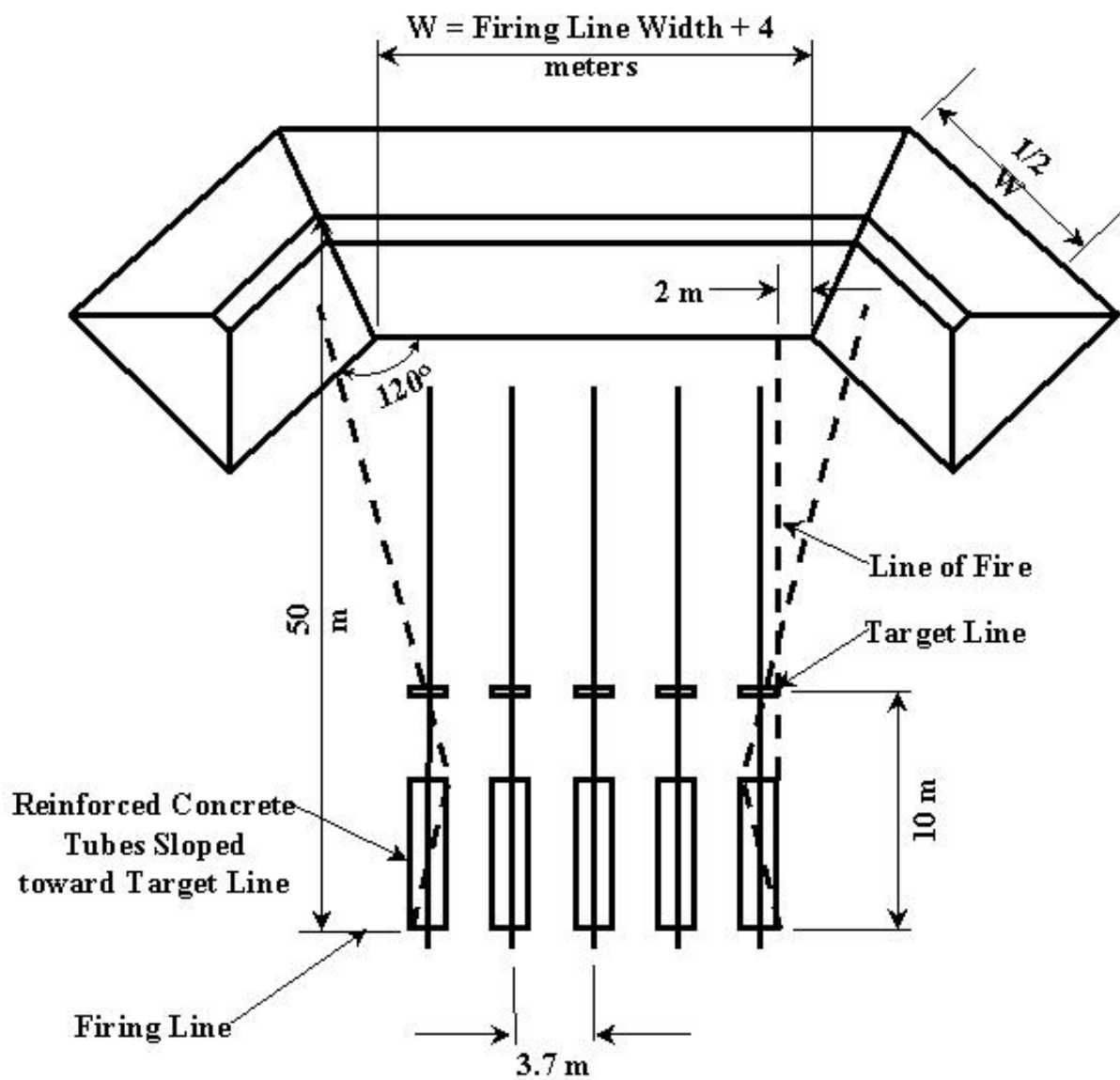
Figure 10. M60 Machine Gun, 10-Meter Tube Range Typical Range Configuration
