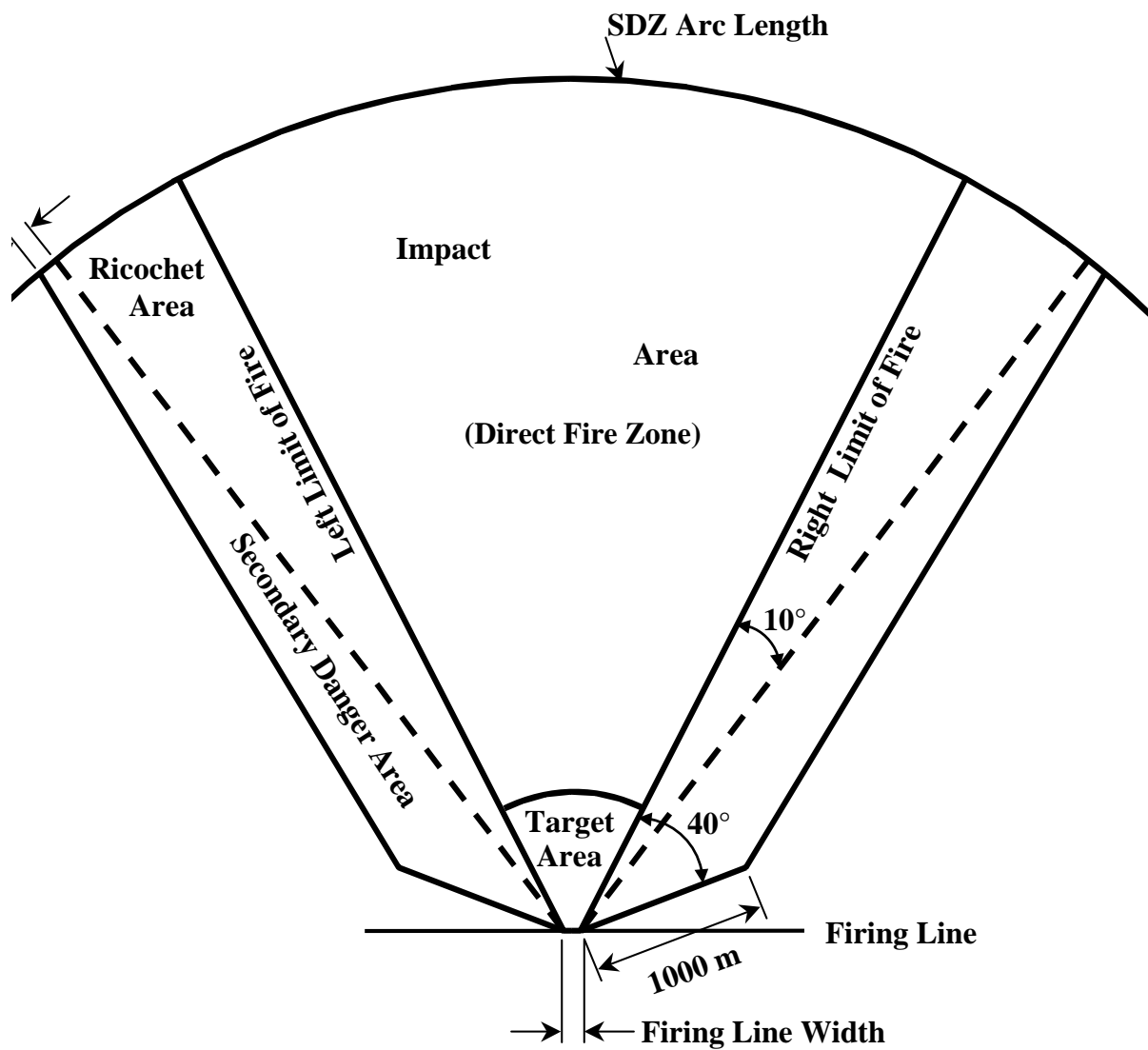
Figure 2. SDZ Configuration — Target Line Wider Than Firing Line
