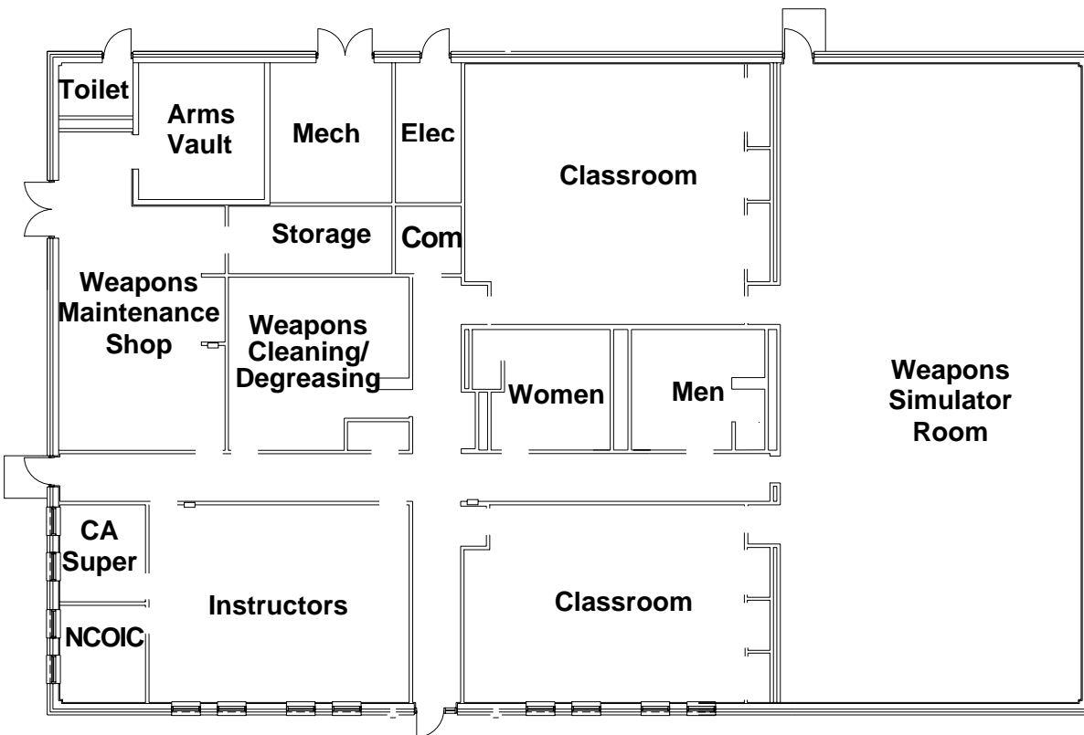
Figure 9. A Typical CA Building Configuration
