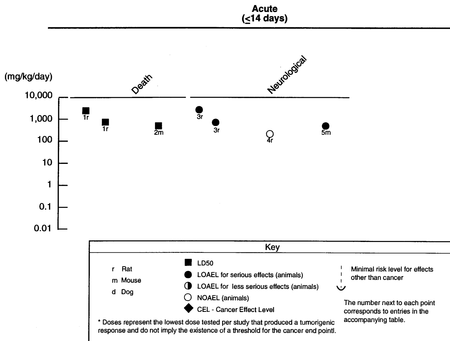
Figure 2-1. Levels of Significant Exposure to 2,4,6-Trinitotoluene – Oral
