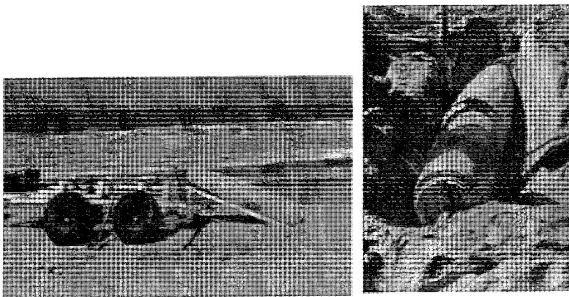
Figure 6.4. Pictures taken during the Mk-63 mine shape emplacement procedure, at low tide, showing the surf zone of Monterey Bay in the background.
