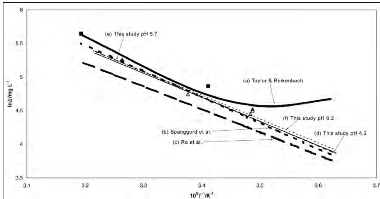
Figure 32. Comparison of TNT solubility literature to this study. (a) Taylor and Rinkenbach (1923); (b) Spanggord et al. (1983); (c) Ro et al. (1996); ■ Gibbs and Popolato (1980); △ Phelan and Barnett (2001); (d) this study pH 4.2 [ \ln(S/\text{mg L}^{-1}) = 16.895 - 3,586.4 K/T , R^2 = 0.9822 ]; (e) this study pH 5.7 [ \ln(S/\text{mg L}^{-1}) = 17.263 - 3,691.3 K/T , R^2 = 0.9837 ]; (f) this study pH 6.2 [ \ln(S/\text{mg L}^{-1}) = 16.777 - 3,542.5 K/T , R^2 = 0.9785 ]
