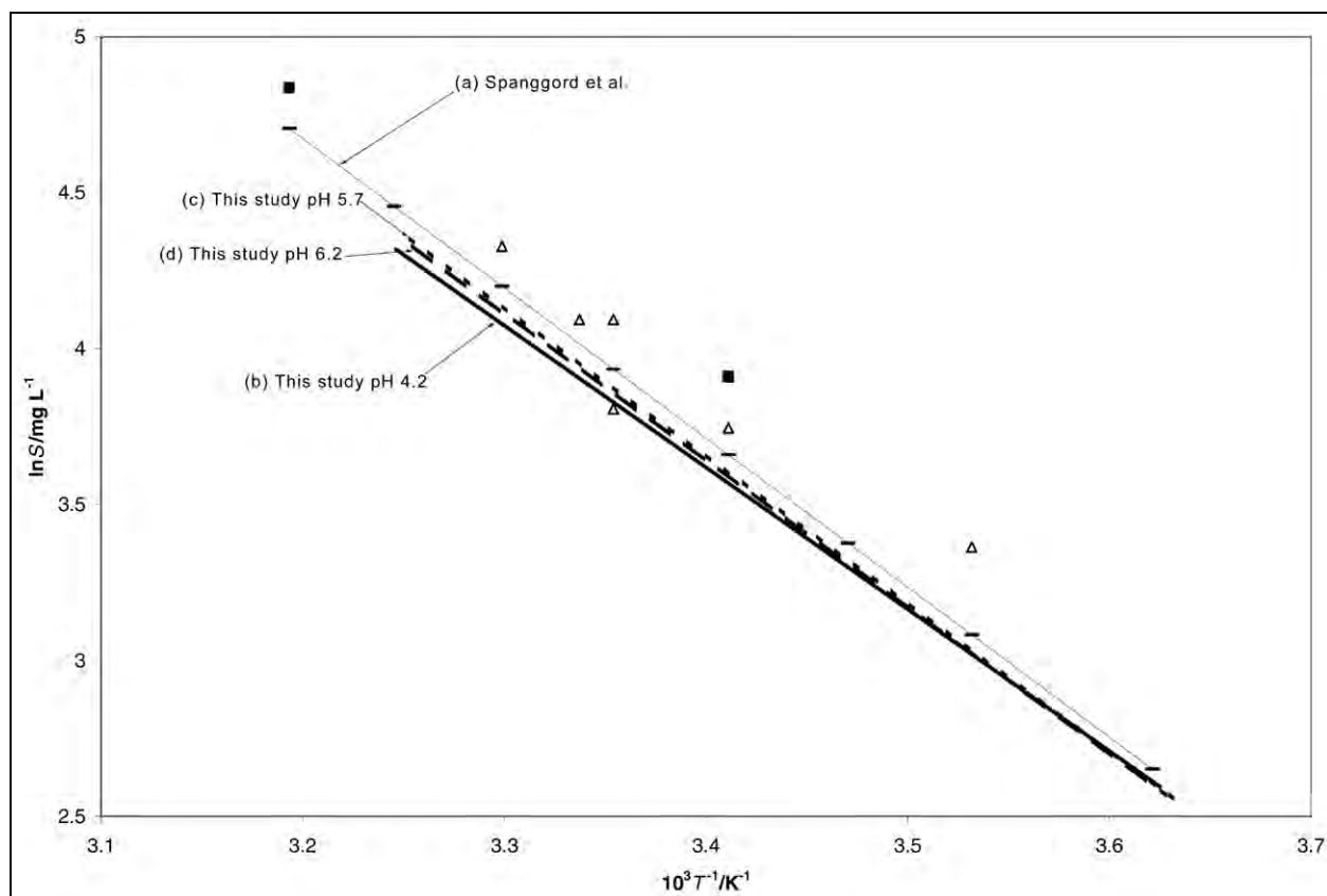
Figure 33. Comparison of RDX solubility literature to this study. (a) Spanggord et al. (1983); ■ Gibbs and Popolato (1980); Δ Townsend and Meyers (1996); (b) this study pH 4.2 [ \ln (S/\text{mg L}^{-1}) = 19.087 - 4,549.1 \text{ K/T} , R^2 = 0.987 ]; (c) this study pH 5.7 [ \ln (S/\text{mg L}^{-1}) = 19.718 - 4,727.8 \text{ K/T} , R^2 = 0.995 ]; (d) this study pH 6.2 [ \ln (S/\text{mg L}^{-1}) = 19.818 - 4,753.2 \text{ K/T} , R^2 = 0.995 ]
