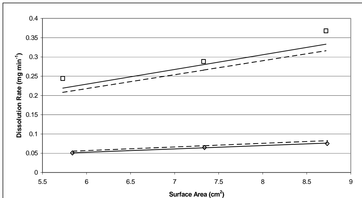
Figure 31. Rate comparisons of TNT study data (□ = 30 °C data, ◇ = 10 °C data) to multiple regression-multiple variable regression line (—) and the Levins and Glastonbury (1972a) regression line (---)
