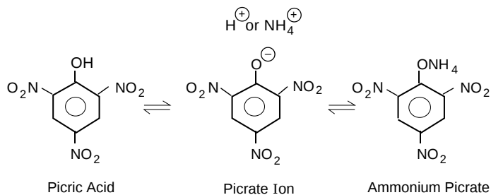
Figure 1. Chemical structures of picric acid, picrate ion and ammonium picrate.
