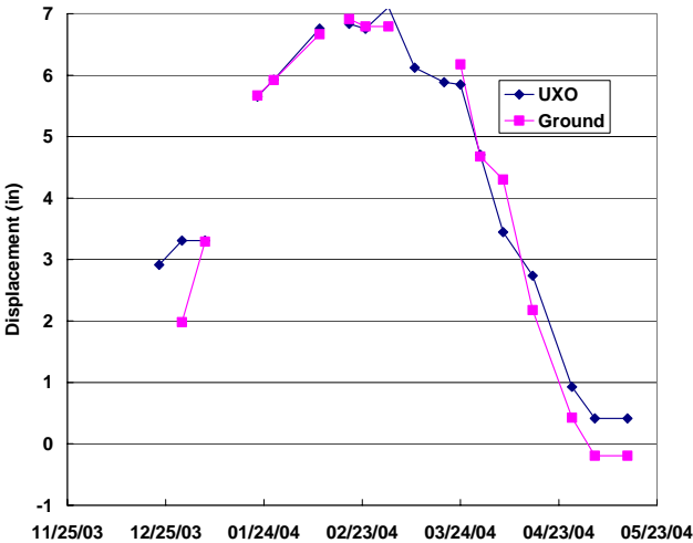
Figure 4. Displacement of surface and 40-mm projectile, buried 4 inches deep, with respect to elevation on 16 Sept. 2003.
