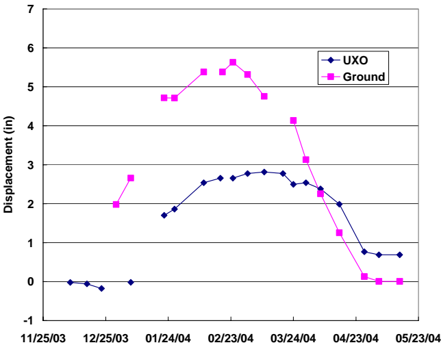
Figure 3. Displacement of surface and 81-mm mortar, buried 24 inches deep, with respect to elevation on 16 Sept. 2003.
