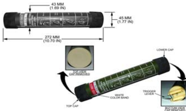
U.K. ILLUMINATION FLARE, CARTRIDGE, PARACHUTE, L5A4
