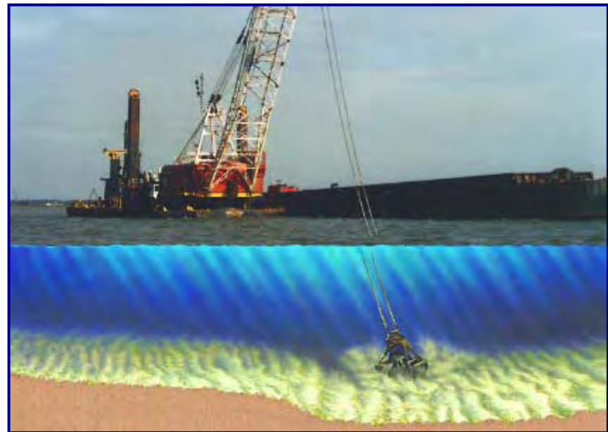
Mechanical Dredging Operation Photo courtesy of U.S. Army Corps of Engineers
