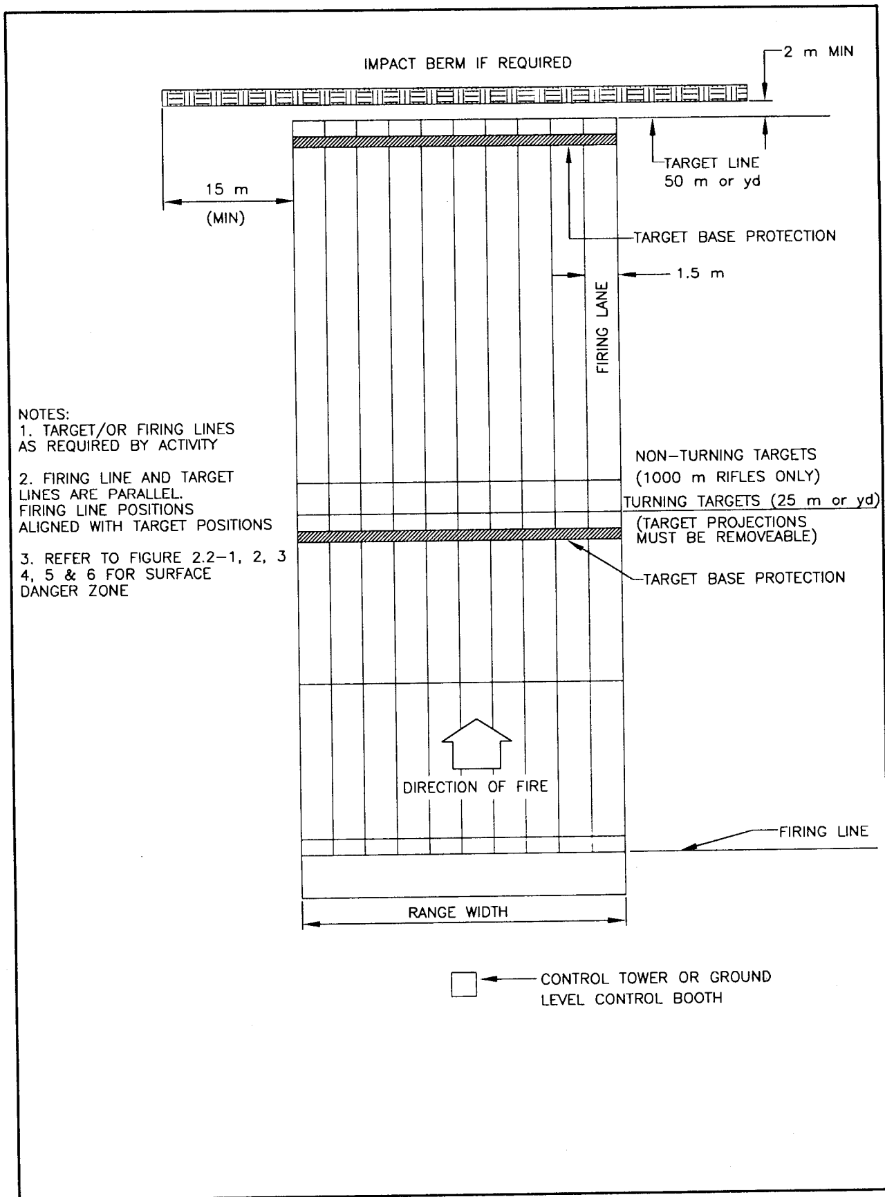
Figure 2.2-7 Outdoor Pistol Range Layout
