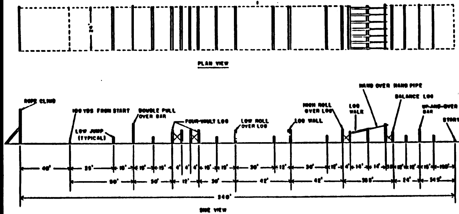
Figure 10 Typical Obstacle Course Layout
