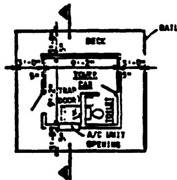
FLOOR PLAN - SPOTTING TOWER
