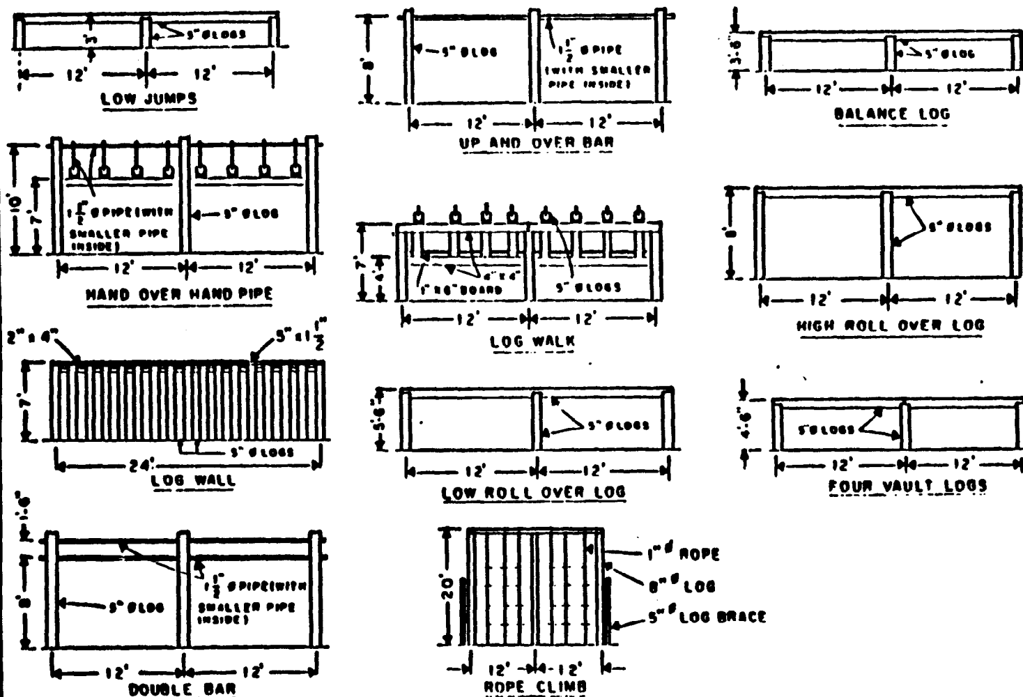
Figure 11 Details of Obstacles
