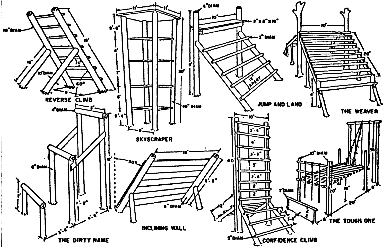
Figure 12 Confidence Course Obstacles
