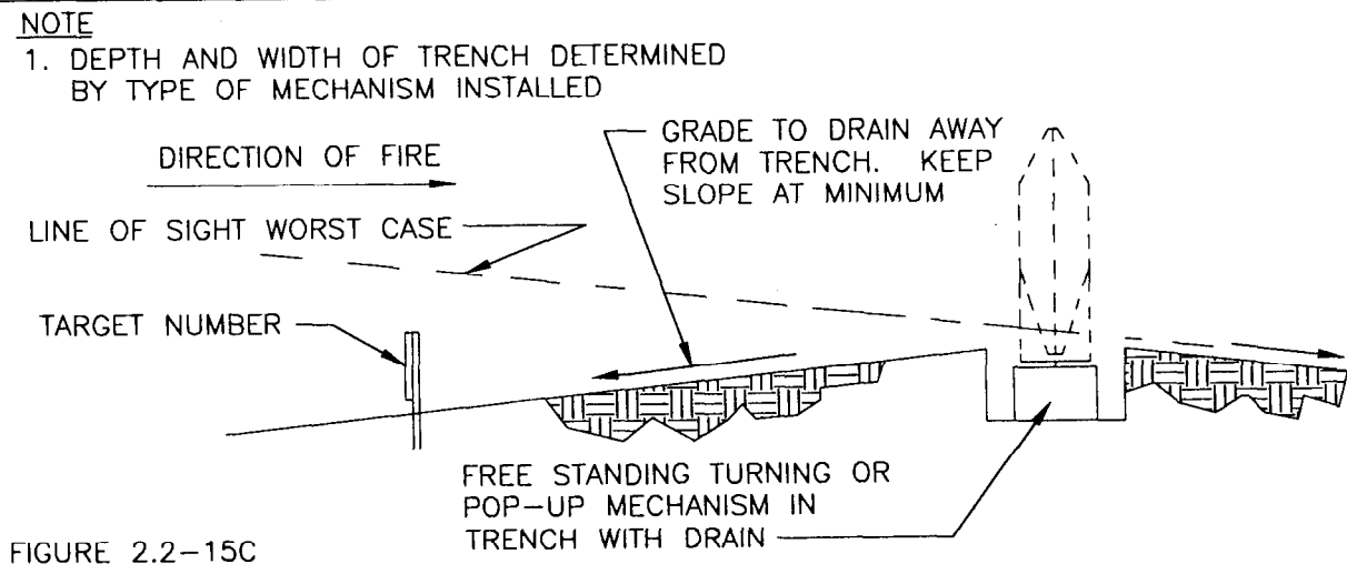
Figure 2.2-15 Ballistic Protection of Target Mechanism
