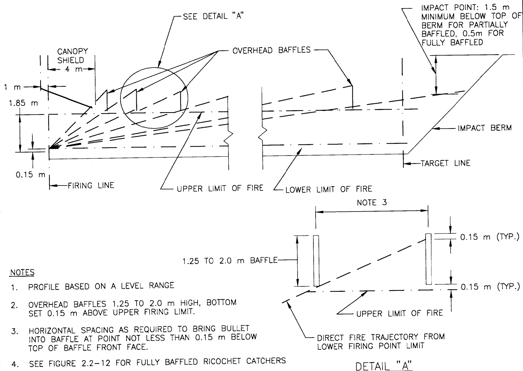
Figure 2.2-9 Baffled Range Profile
