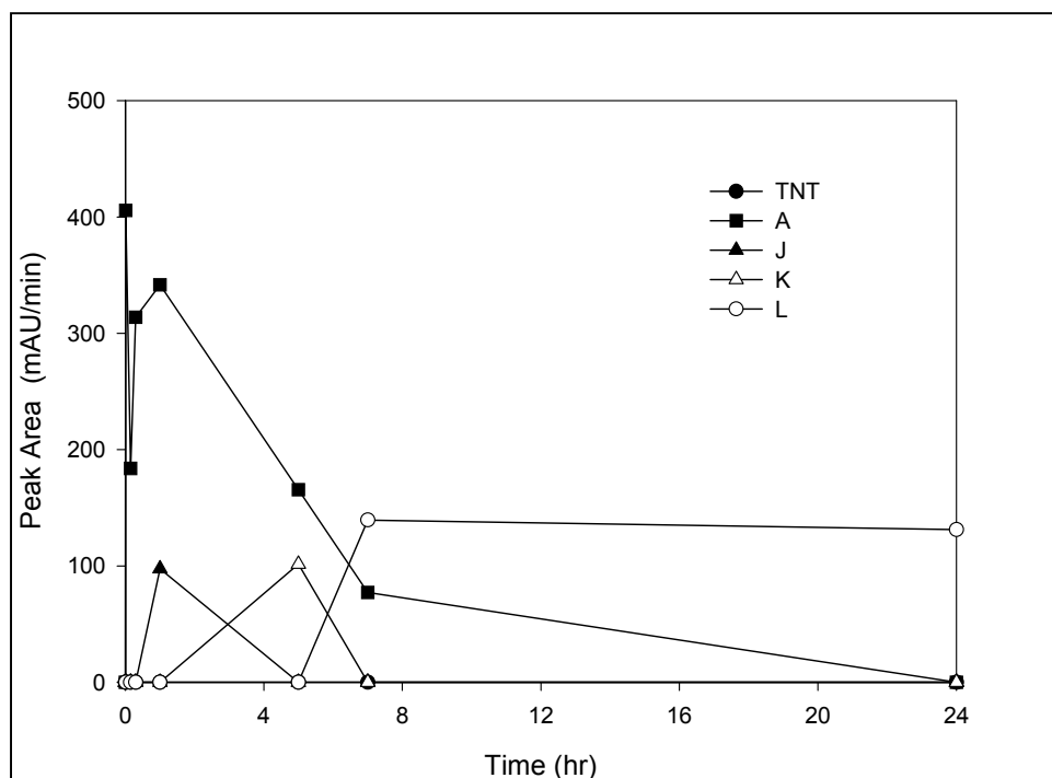
Figure 1. TNT transformation product formation and disappearance
