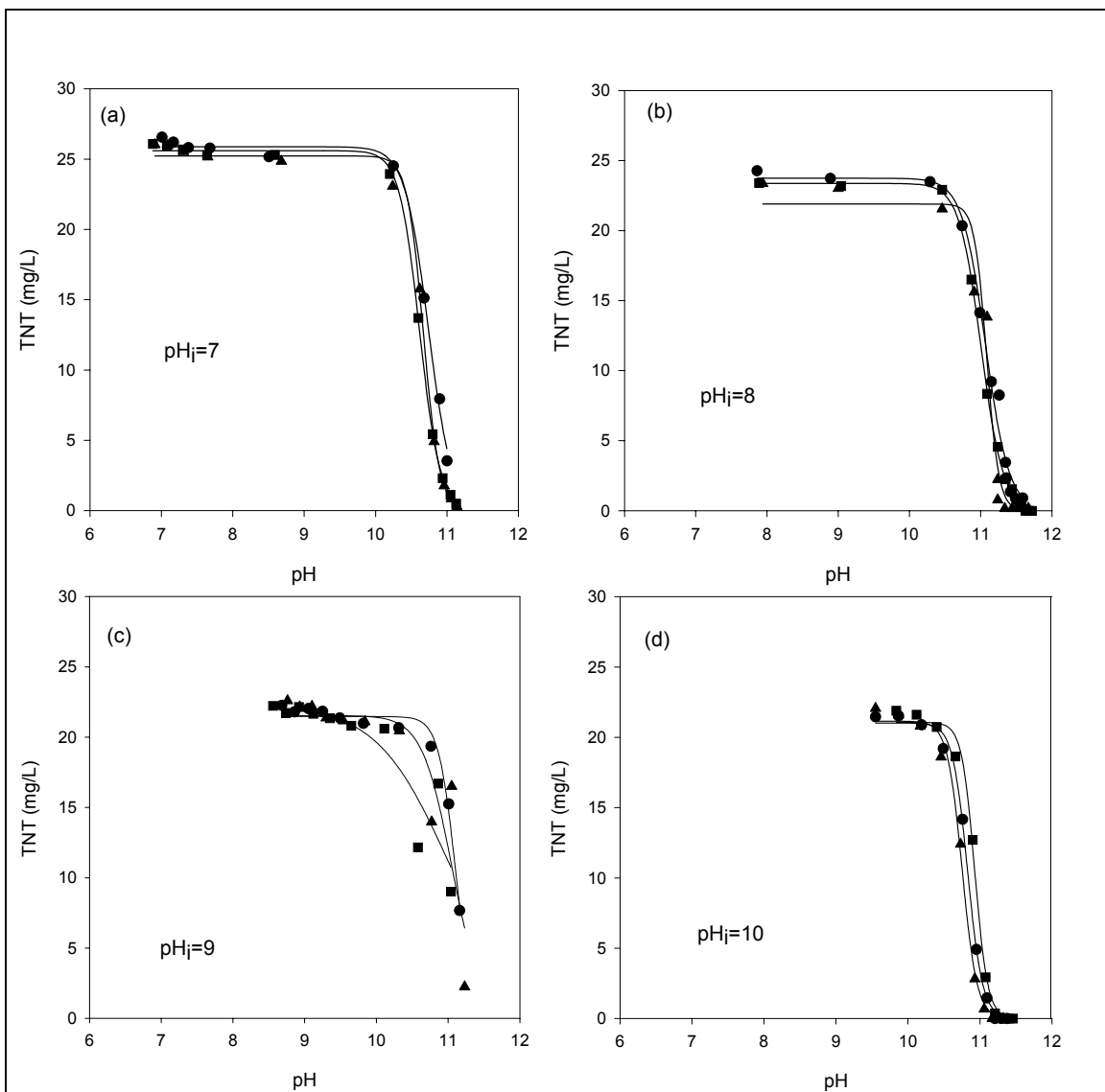
Figure 5. Titration curves of various buffered TNT solutions
