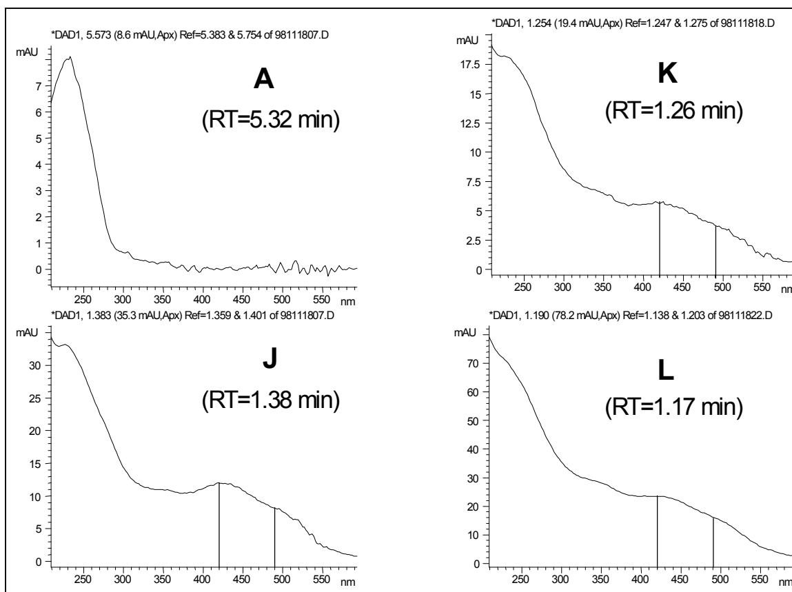
Figure 2. UV spectra of unidentified intermediates
