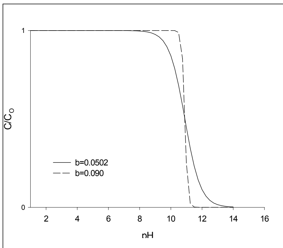
Figure 6. Parametric analysis of TNT removal model
