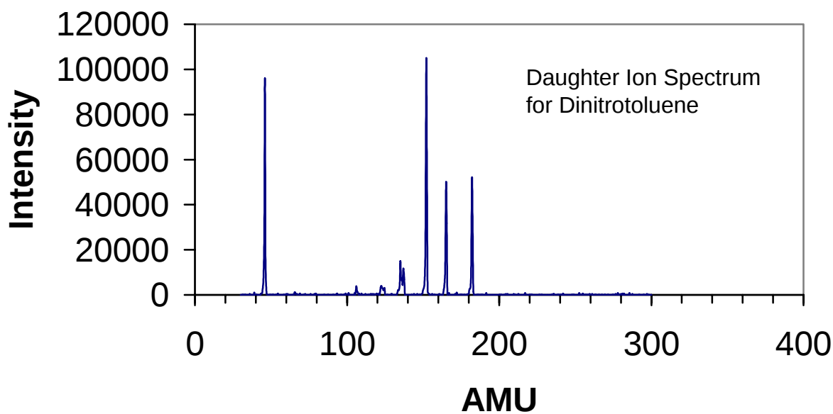
Figure A-6. Daughter Ion Spectrum for Dinitrotoluene
