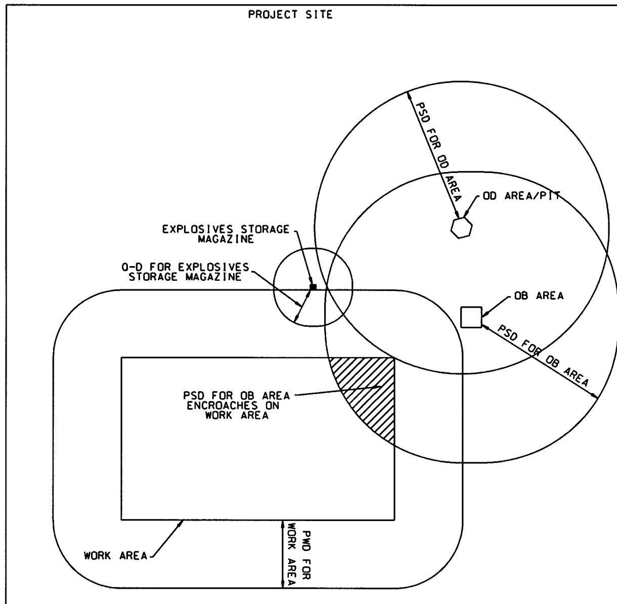
FIGURE 5-2: SAMPLE OF A Q-D MAP FOR A PROJECT SITE WITH ENCROACHING PSD
