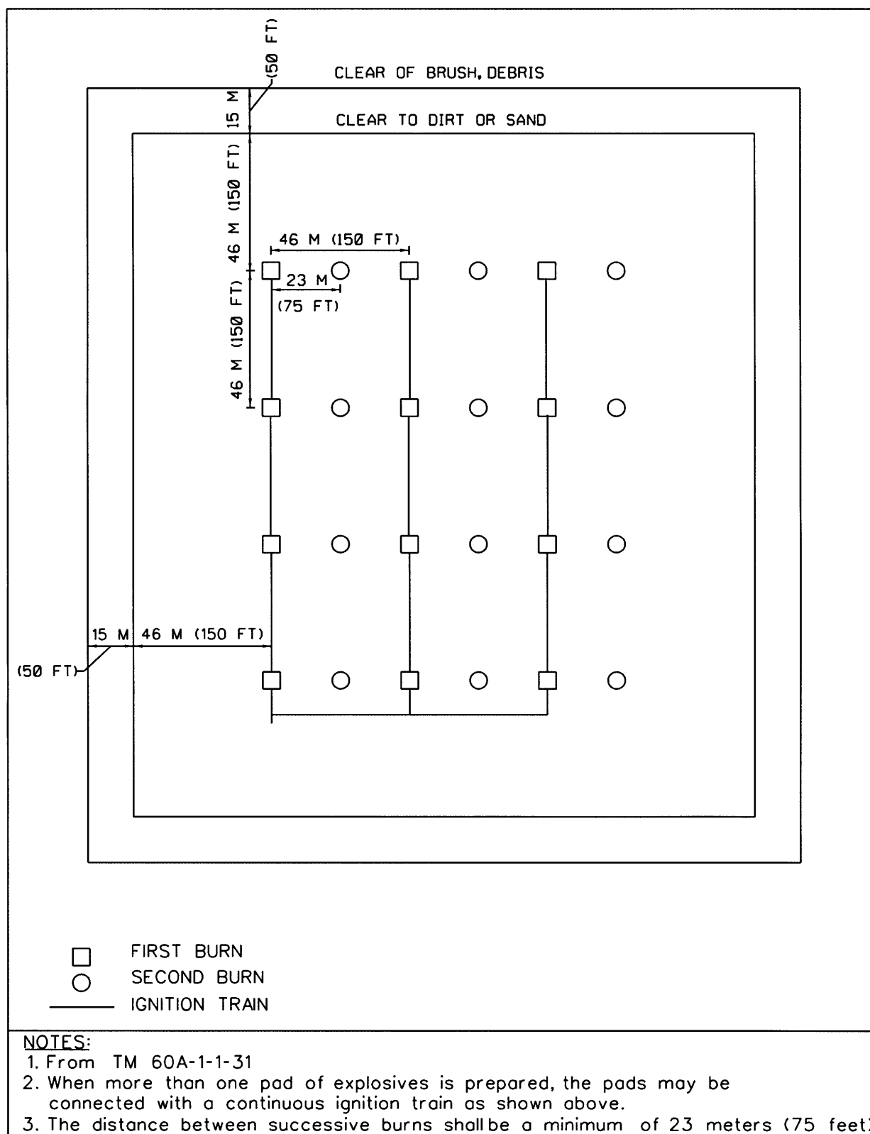
FIGURE 3-6: TYPICAL SURFACE BURNING AREA
