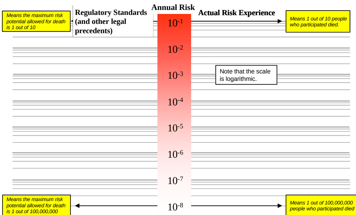
Figure 10: URS Format
