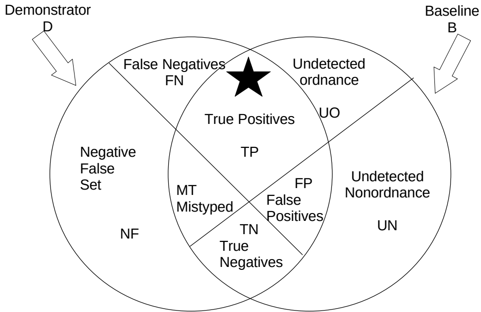
Figure 1. Venn Diagram
