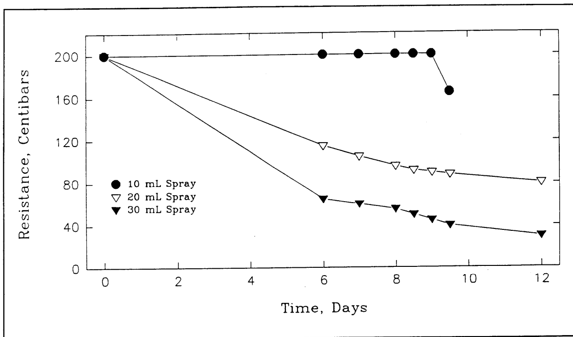
Figure 11. Time required for 10, 20, and 30 mL volumes of water to reach the moisture probe in the static cell following spray application (Resistance decreases as moisture approaches the probe.)
