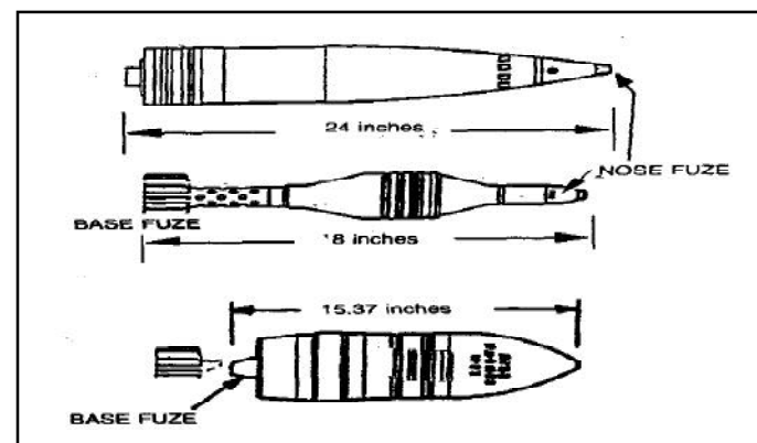
Figure 5. Typical Projectiles.
