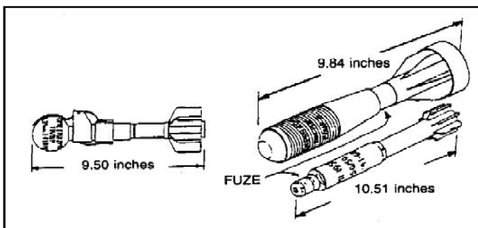
Figure 8. Rifle Grenades.
